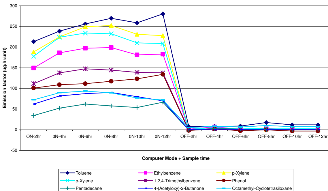
Figure 1 IVOCs Emission factor for computer 2 (an example for “active” sources)
