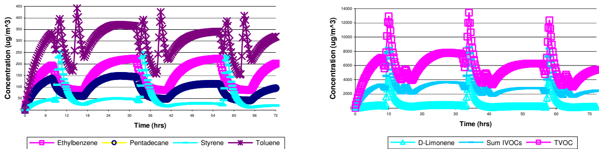
Figure 3 Impacts of emissions of tested sources on VOC concentrations in a typical office environment
