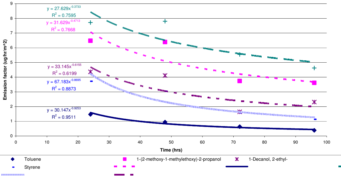
Figure 2 IVOCs Emission factor for carpet test (an example for “passive” sources)
